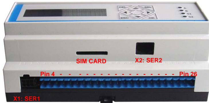
Bottom-side view
