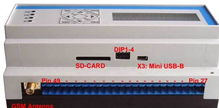
Top-side view
